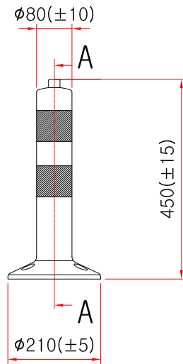
SIDE ELEVATION SCALE : NONE
